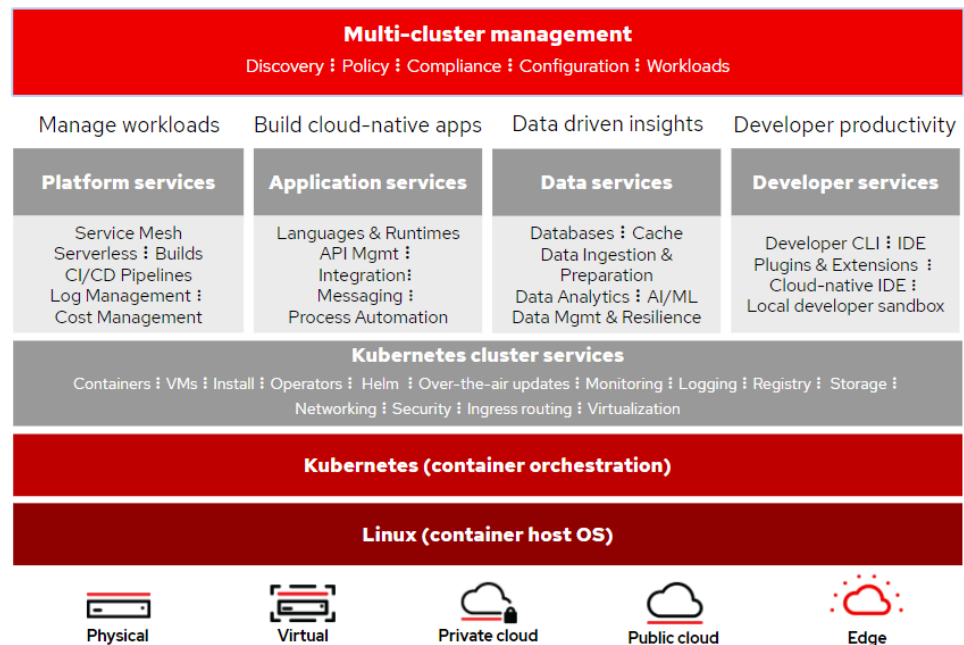
Figure 1. Red Hat OpenShift architecture overview
